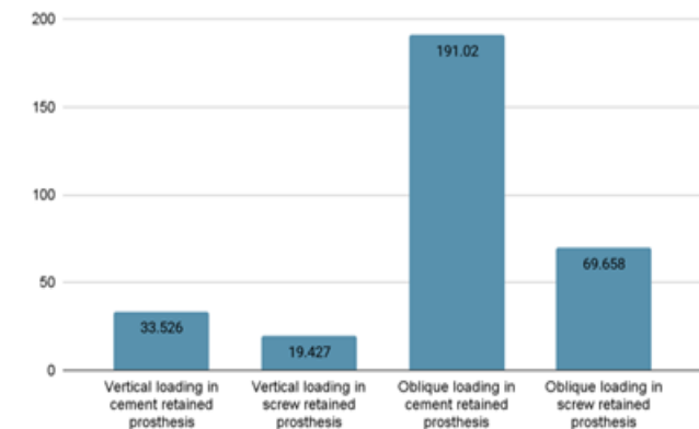
Graph 2: von Mises stress in dental implant restored with cement and screw retained PFM crown in vertical loading of 100N and oblique loading of 100N.
